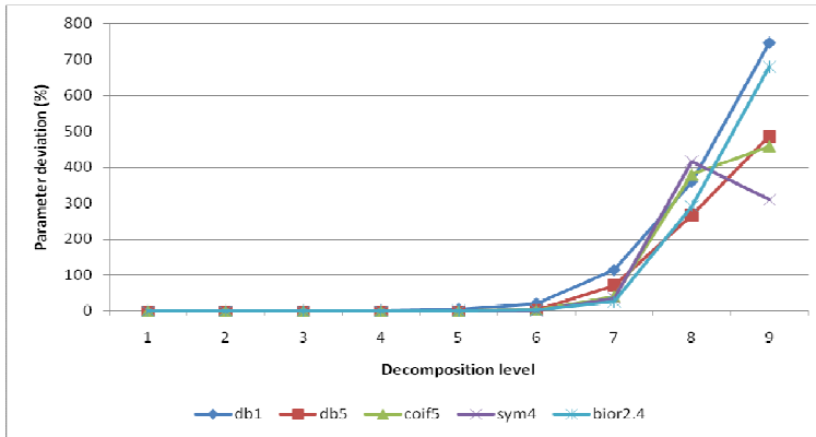
Fig. 3 Relative changes in Z_{sk} during wavelet approximation for roundness profiles (sample: n = 100 profiles).
